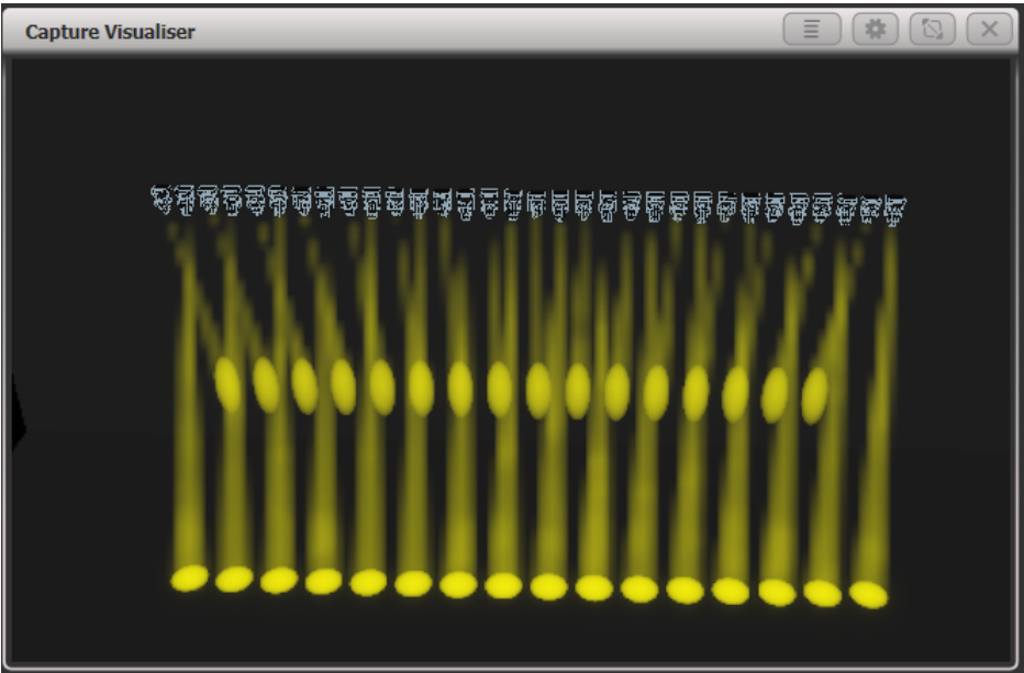
Spread = 2 (Phase = 180 degrees):
